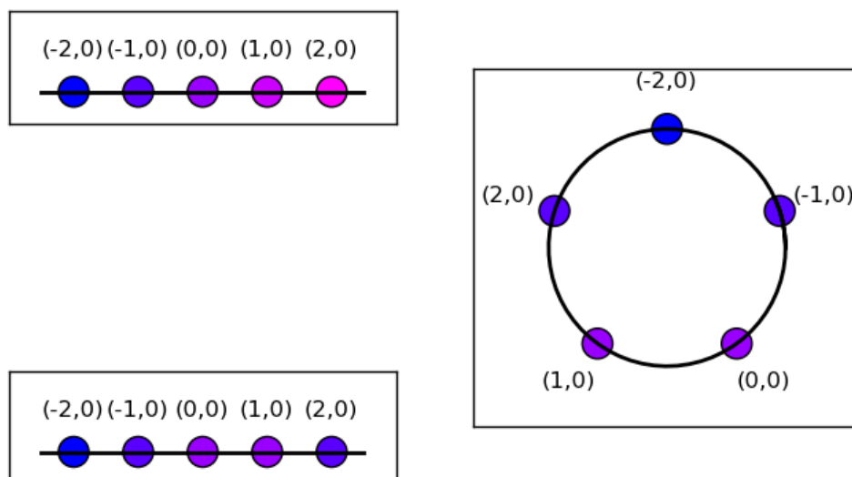
Figure 2.5: Top left: Layer with single row and five columns without periodic boundary conditions. Numbers above elements show element coordinates. Colors shifting from blue to magenta mark increasing distance from the element at (-2,0) . Bottom left: Same layer, but with periodic boundary conditions. Note that the element at (2,0) now is a nearest neighbor to the element at (-2,0) . Right: Layer with periodic boundary condition arranged on a circle to illustrate neighborhood relationships.
